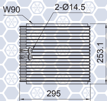
F2-00763 CAMRY / ES300
