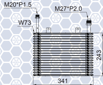
FA-00783 CARAVAN (FRONT UNIT) / TOWN & COUNTRY (FRONT UNIT) / VOYAGER (FRONT UNIT)
