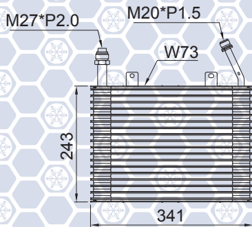
F8-00766 BLAZER ST P/U / JIMMY ST / ST PICK UP
