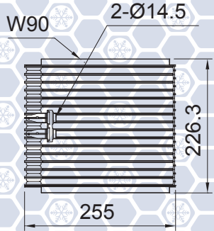
F2-00757 STARLET / TERCEL
