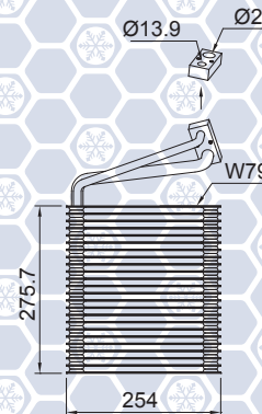
FA-00783 CARAVAN (FRONT UNIT) / TOWN & COUNTRY (FRONT UNIT) / VOYAGER (FRONT UNIT)
