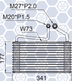
F8-00918 CIELO R134A / RACER R134A
