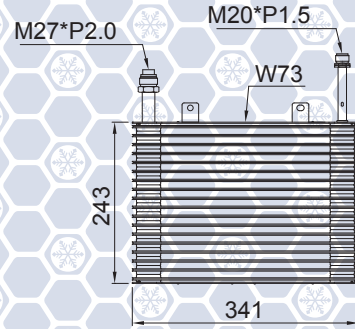
F8-00923 BLAZER R134A
